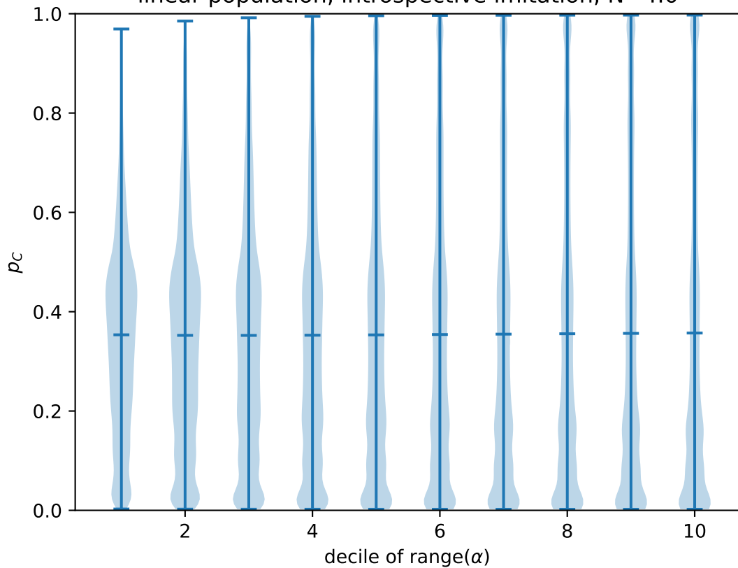
linear population, introspective imitation, N=4.0
